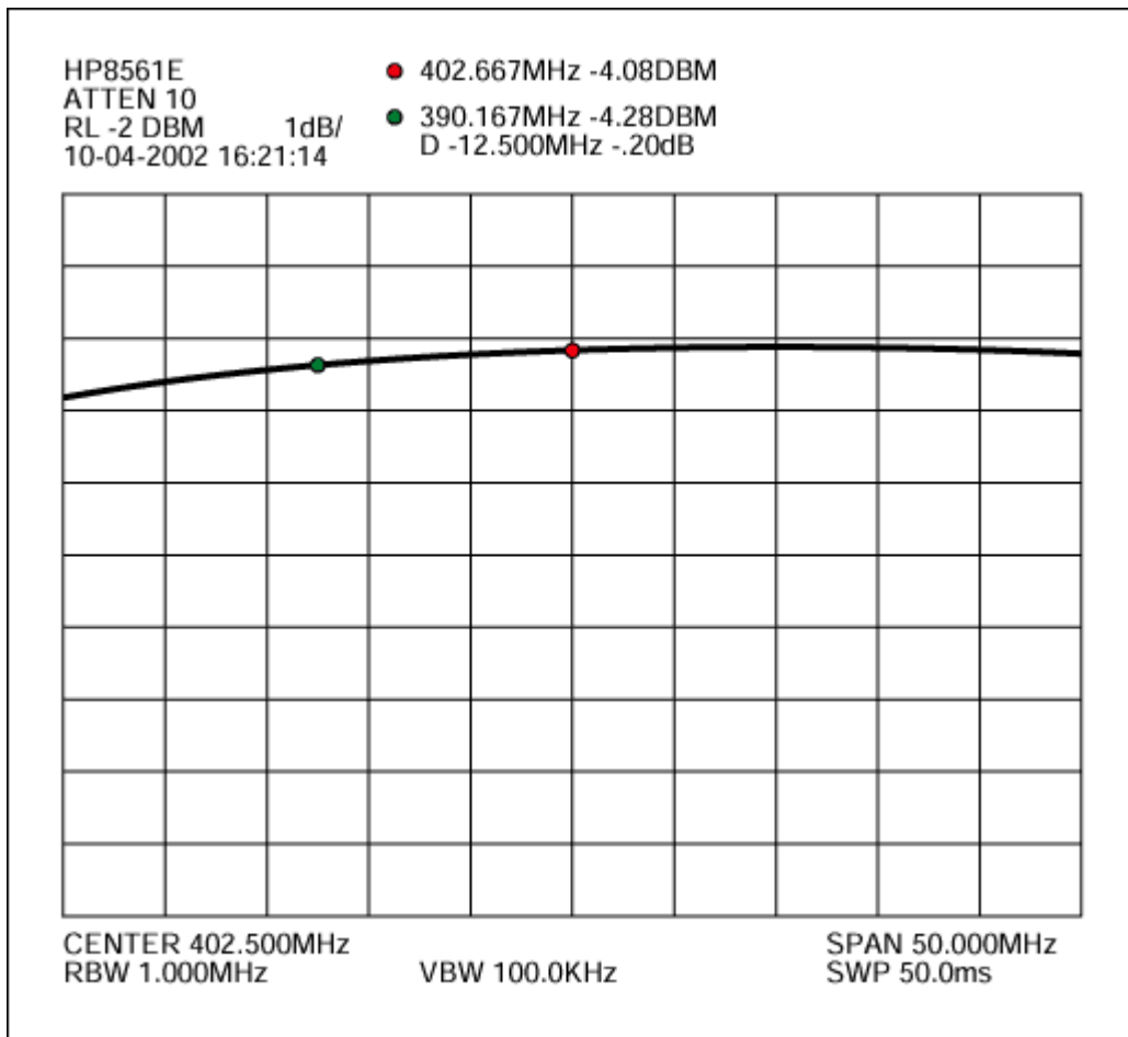
Figure 7. Gain flatness
